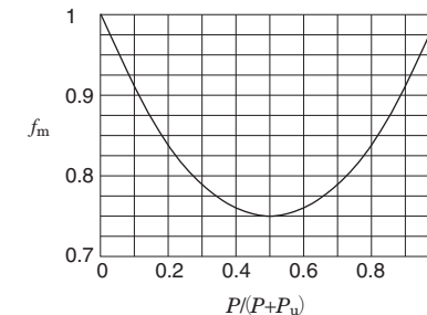
Fig. 5-12 Coefficient f_m
