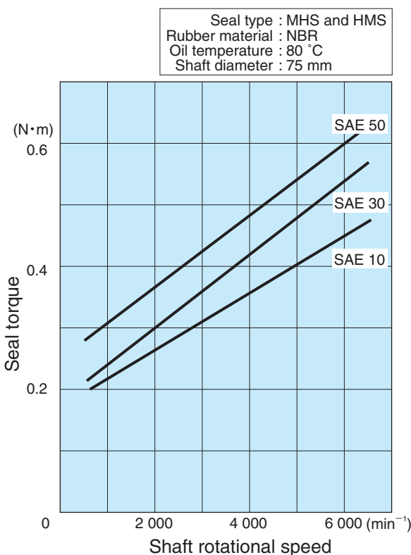
Fig. 1.6.10 Relation between rotational speed and seal torque
