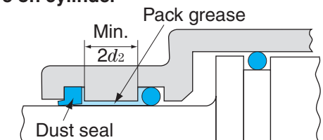
Fig. 2.4.2 Typical installation of O-ring for dynamic sealing
