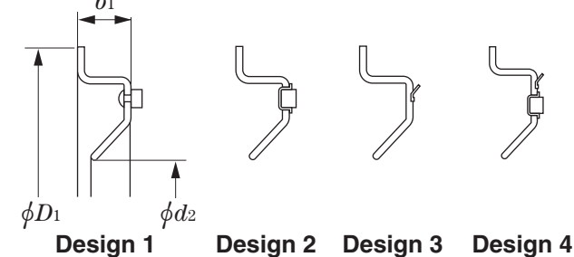
Seal inner rings
