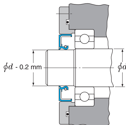
Fig. 1.7.3 Recommended shaft profile and machine construction to avoid damaging shaft surface
