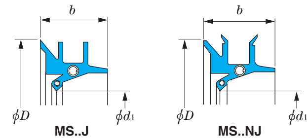
MORGOIL seals
