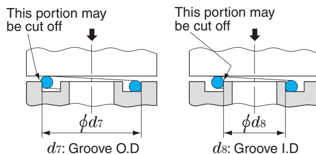
For internal pressure For external pressure
