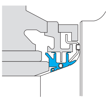
Mounting example
